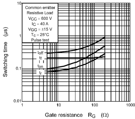
Fig. 8.10 Switching Time - R_G
