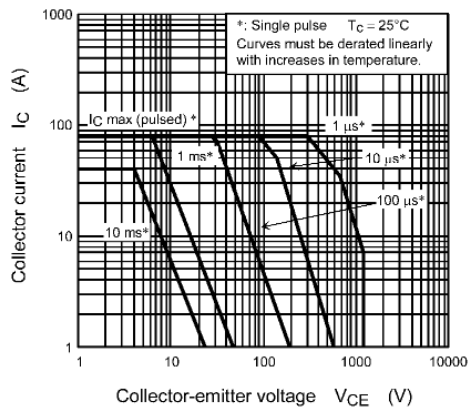
Fig. 8.12 Safe Operating Area (Guaranteed Maximum)
