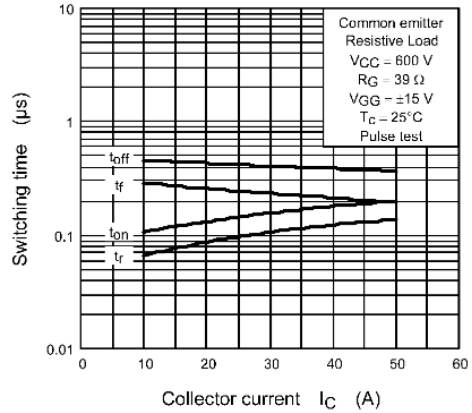
Fig. 8.9 Switching Time - I_C
