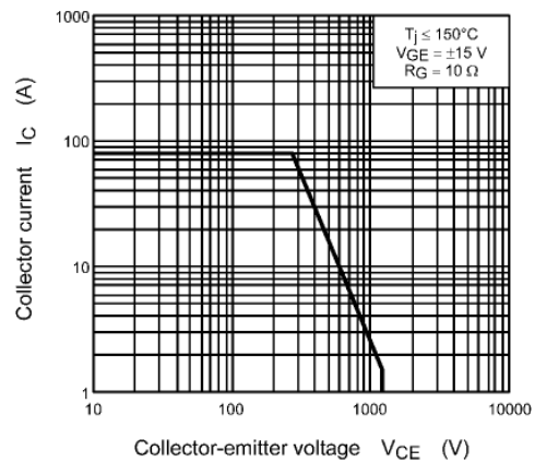
Fig. 8.13 Reverse Bias SOA (Guaranteed Maximum)
