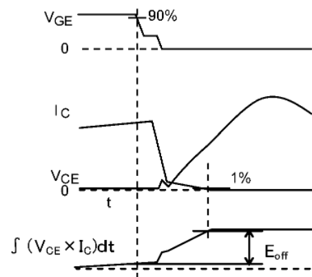
Fig. 6.2.4 Timing Chart of Switching Loss
